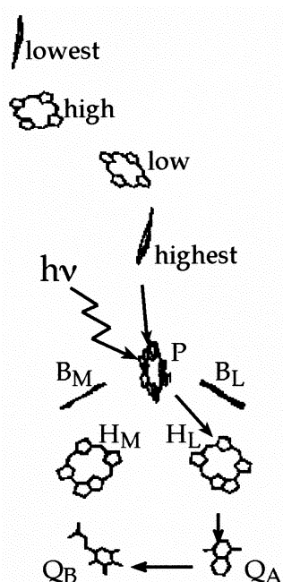
Fig. 6. The position of the redox cofactors in reaction centers of the purple photosynthetic bacteria Rps. viridis . The four hemes are labeled by their relative electrochemical redox potential. The subunit binding the four hemes extends into the periplasmic space. The heme subunit is missing from the Rb. sphaeroides RCs. The rest of the cofactors are within the membrane in RCs from both bacteria. The arrows show the direction of electron transfer. P is a bacteriochlorophyll dimer, B L and B M are bacteriochlorophyll monomers, H L and H M bacteriopheophytins, and Q A and Q B are quinones.
